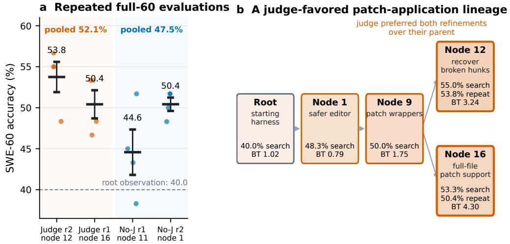
Figure 7: SWE-60 repeatability and a qualitative judged lineage. Left: individual full-60 evaluations of the four selected agents; horizontal markers show means and error bars show standard errors, and the dashed line marks the single 40.0% root observation. Right: one lineage favored during judge-guided search. Stored search-time BT strengths are shown alongside search accuracy; the two selected descendants additionally show their four-evaluation means.
