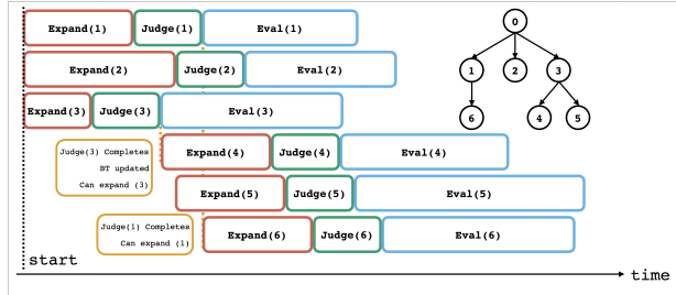
Figure 2: Illustration of the disaggregated pipeline. SIFT allows expansions of nodes that have yet to complete full evaluation but received a strong signal from the judge.
