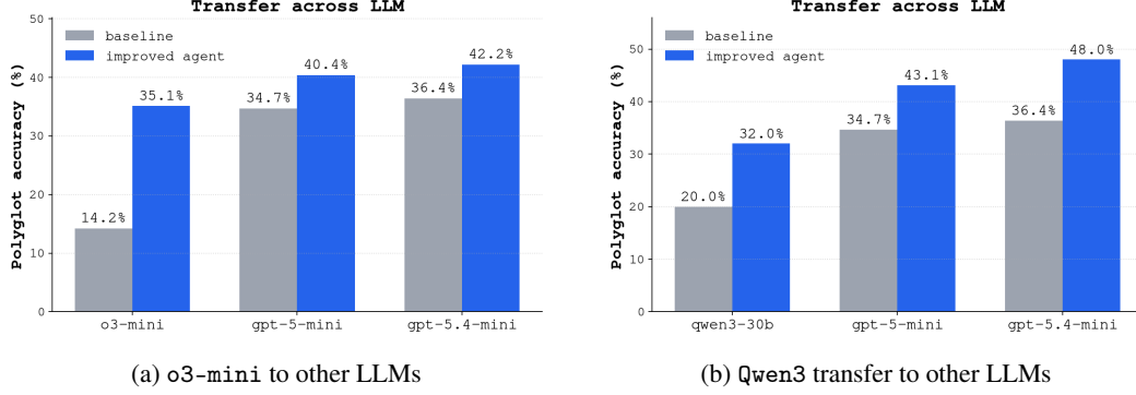
Figure 4: Transfer between LLMs of the best Polyglot agent found by SIFT. The improved agents in SIFT generalizes to gpt-5-mini and gpt-5.4-mini, where the improved agent consistently achieves a higher accuracy than the base coding agent.
