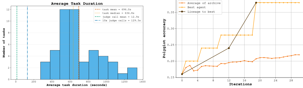
(a) Task duration distribution on Polyglot. The average set of pairwise judge comparisons against the top 10 incumbent patches complete in a significantly shorter period of time than even the first evaluation.
