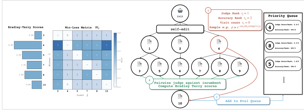
Figure 1: Illustration of the SIFT pipeline. In a single expansion step, node i is sampled with probability P(i) \propto \exp(-(\alpha r_b(i) + \beta r_a(i) + \eta \log(1 + v_i))) , self-improves, then judged against previous versions in the existing agent archive. The win/loss record is updated and the BT scores of each node is solved numerically. Then the new agent is inserted into the priority queue for evaluation on downstream tasks, prioritizing higher potential nodes.
