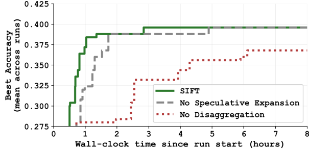
Figure 5: Speedups in SIFT, averaged across five runs.
