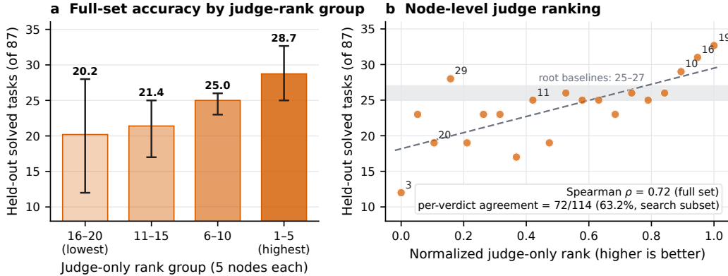
Figure 8: TerminalBench judge ranking versus held-out full-set performance for all 20 fully evaluated candidates in the judged run. Every candidate was evaluated once on the full 87-task set under the rerun protocol; the two final picks (nodes 19 and 11) use their three-evaluation means. Left: nodes are sorted by judge-only Bradley–Terry rank and divided into four consecutive groups of five; bars show each group’s mean full-set score and whiskers cover the min–max range of its five nodes. Mean accuracy rises monotonically from 20.2/87 for judge ranks 16–20 to 28.7/87 for ranks 1–5. Right: the underlying node-level judge rank versus full-set score; the shaded band covers the starting agent’s three baseline evaluations (25–27). Per-verdict agreement excludes equal-score pairs; the BT fit uses only actual LLM verdicts (order-split comparisons abstain) and excludes synthetic smoke-gate wins.
